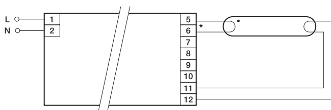
EcoTronic 18–58W
